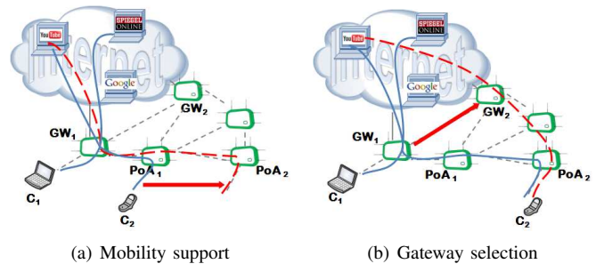
Fig. 1. Mobility support and resource management in wireless mesh networks
