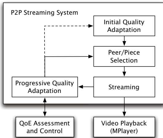
Fig. 3. Quality adaptive P2P streaming system architecture.
